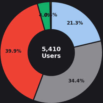
Persona Distribution
